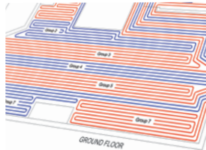
Example of a layout plan
